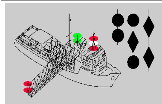
Vessel engaged in dredging or underwater operations when restricted in ability to maneuver & not making way. Mnemonic, Diamonds are a girl's best friend; don't bust your Balls between the ship and the shore.
