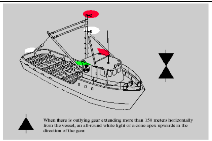
Vessel engaged in Fishing, other than Trawling, Making Way. Mnemonic, Red over White Fishing Tonight
