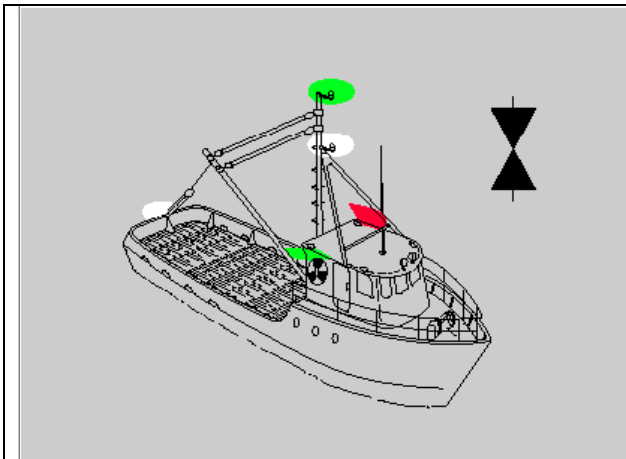
Trawler Making Way. Vessel < 50 meters in length. Mnemonic, Green over White Trawling Tonight
