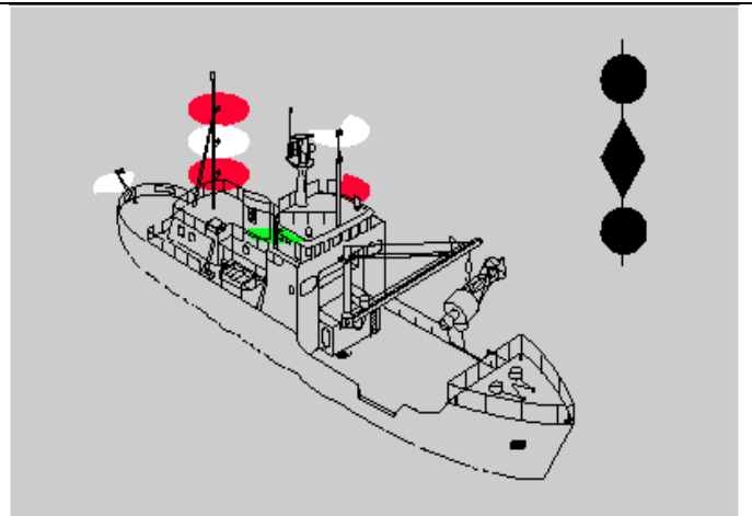
Vessel restricted in her ability to maneuver & Making Way. Vessel < 50 meters in length.
